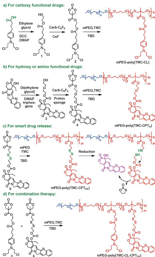
Scheme 2. Detailed synthetic routes of polymerizable prodrugs and their polymers.
